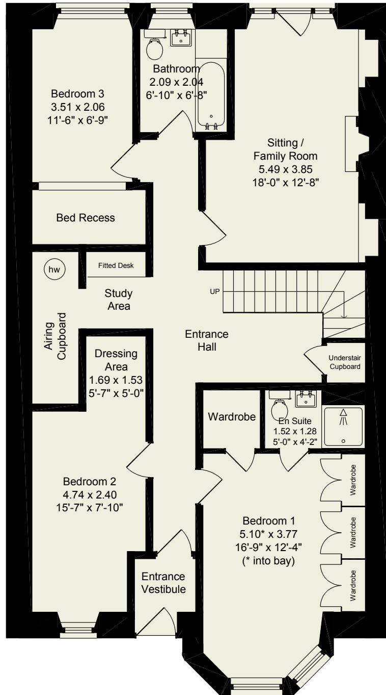
Garden Level
